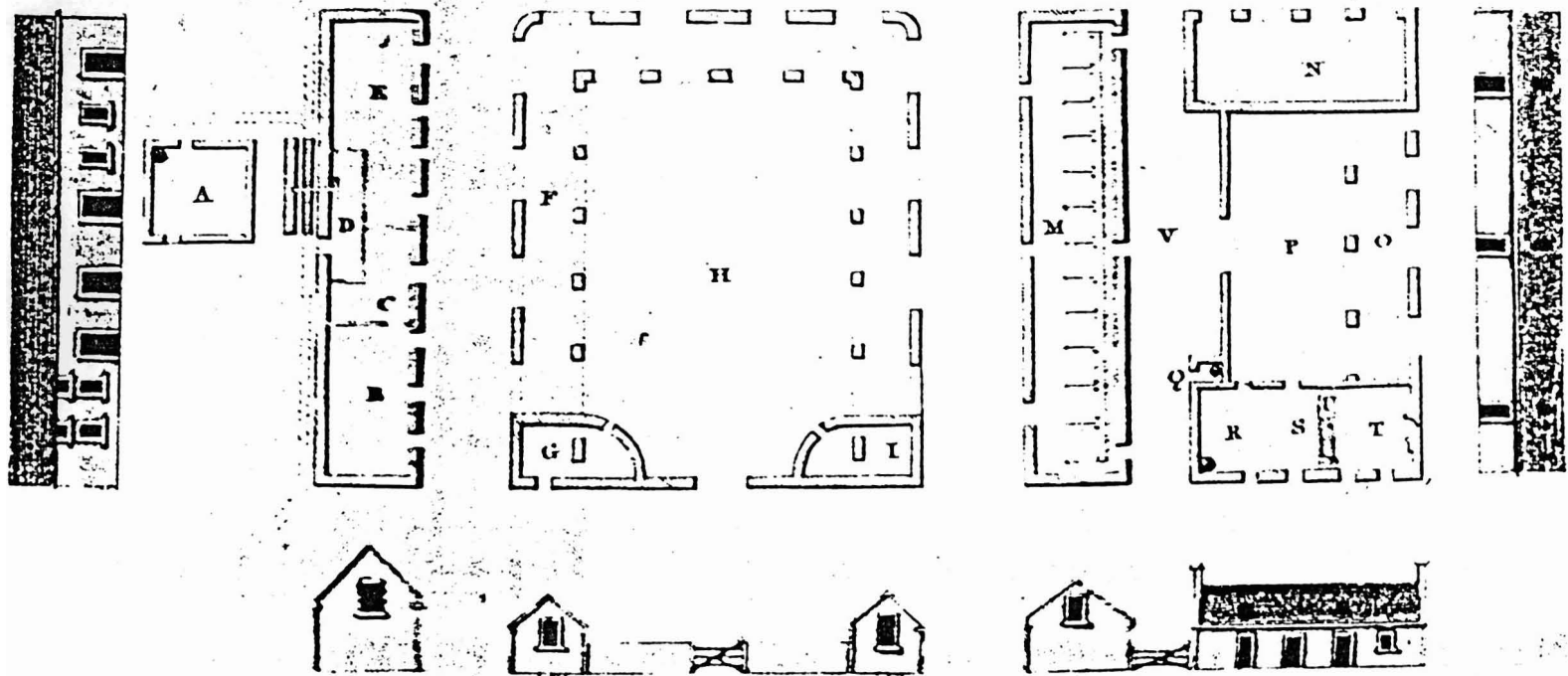
Fig. 90. Skelbo, Dornoch, Sutherland: 1812. A single-storey steading with 1 1/2-storey barn wing to west. Note that the byres have trevises between every second animal as was common later and that there is a feeding passage at the animals' heads. This is a feature that normally only occurs on the most elaborate plans. (NMA: C3981)
